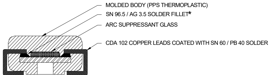
SECTIONAL VIEW
