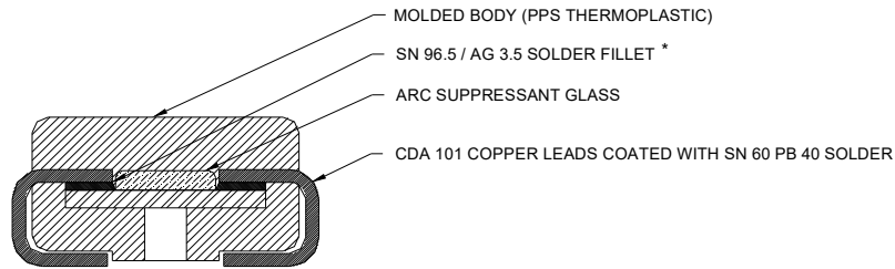
SECTIONAL VIEW
