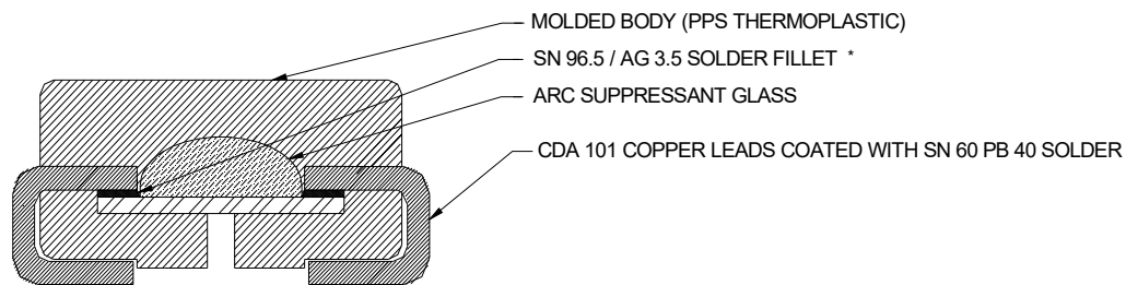
SECTIONAL VIEW
