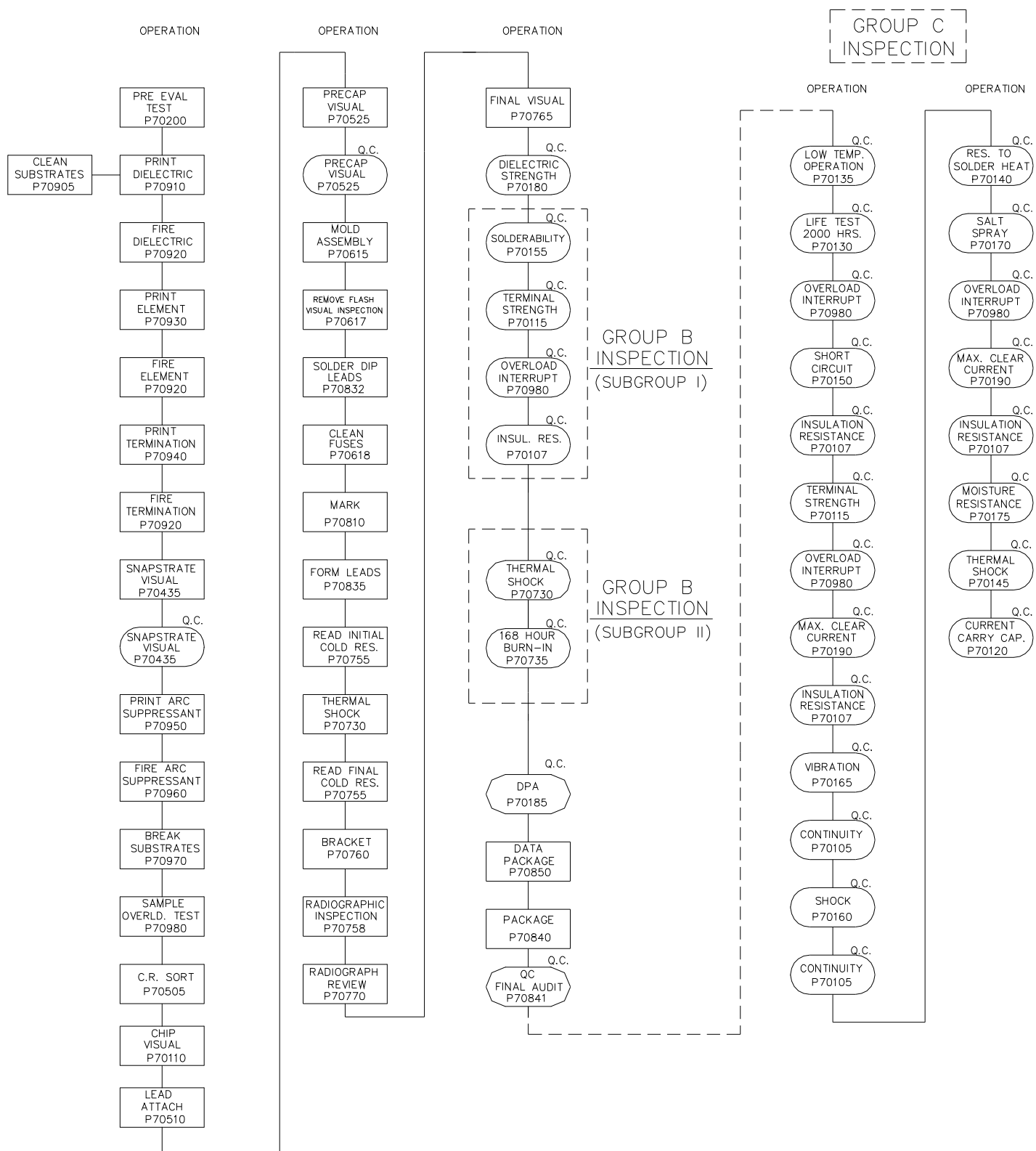
FIGURE 6 OPERATIONS FLOW CHART
